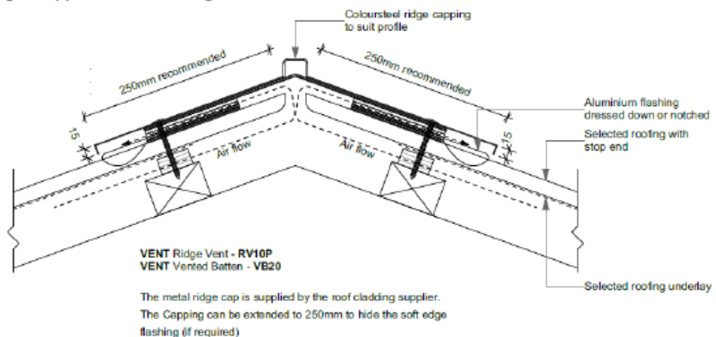
Fig E: Application with Ridge Vent
