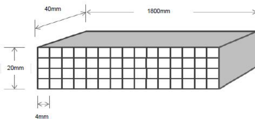
Fig C: Dimensions
