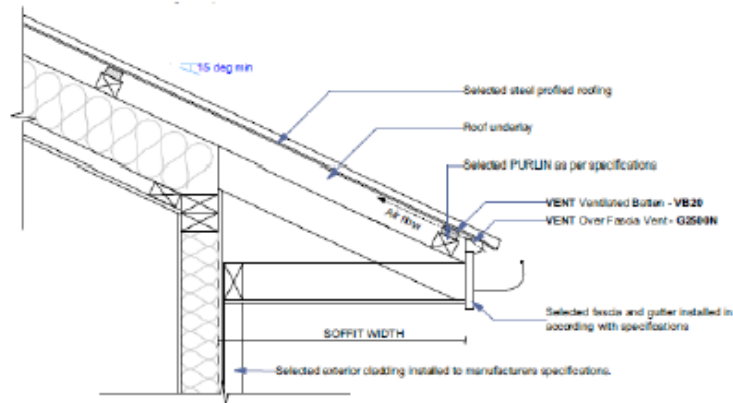
Fig D: Application on purlins
