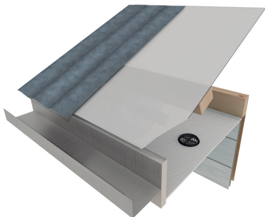
Fig C: Circular Soffit Vent G700
