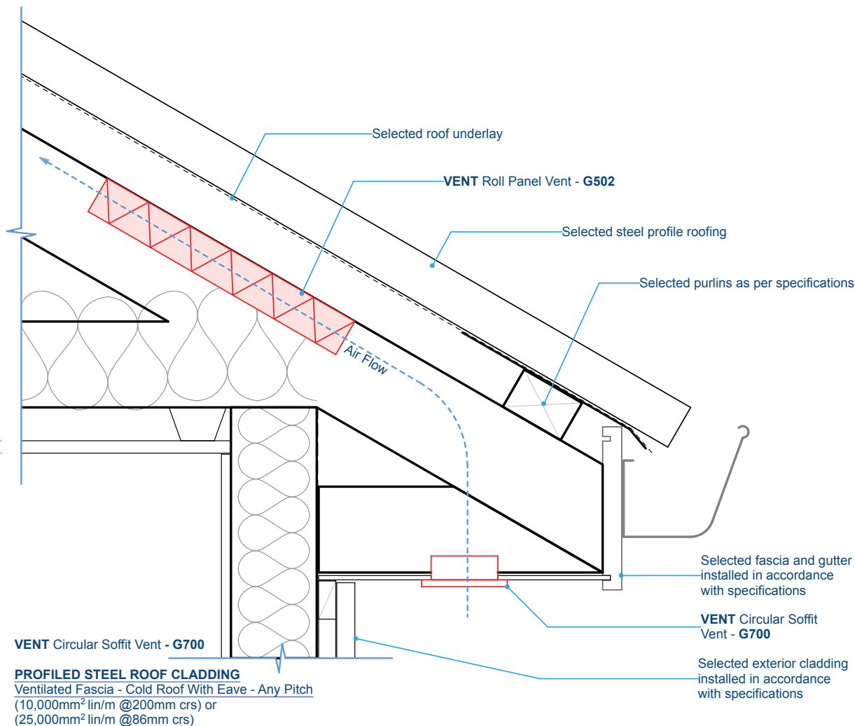
Fig B: Trussed Roof Application
