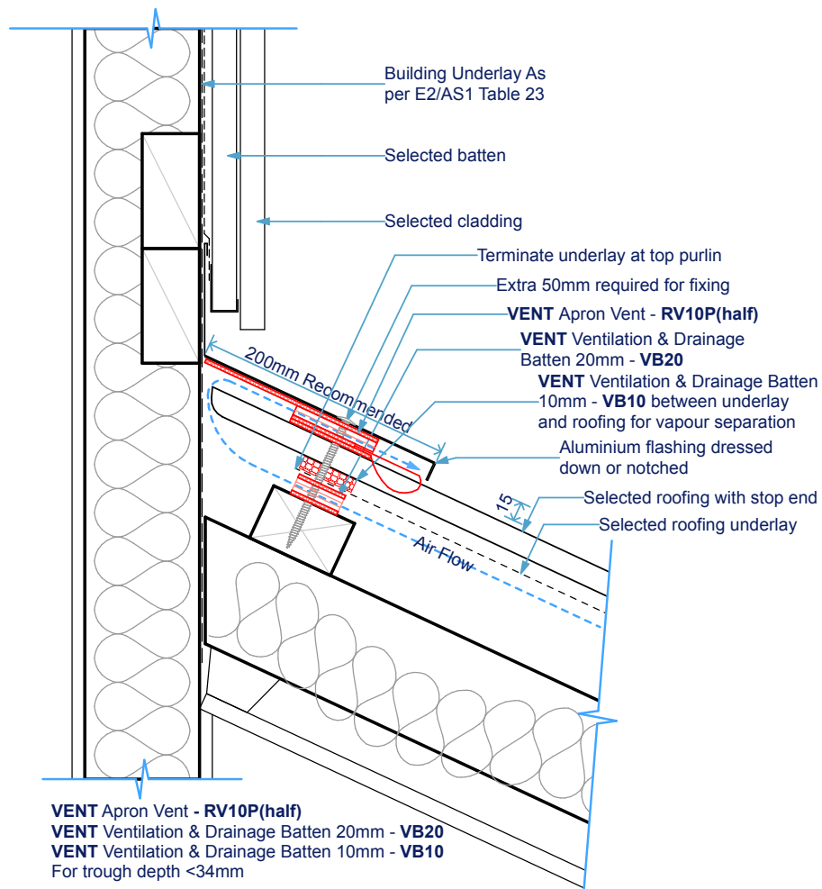
Fig A: Skillion Roof Abutment Application
