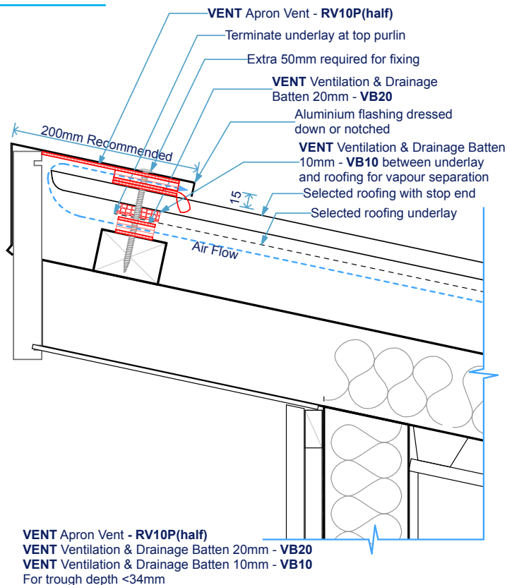
PROFILED STEEL ROOF CLADDING Ventilated Ridge Barge Detail - Skillion Roof
